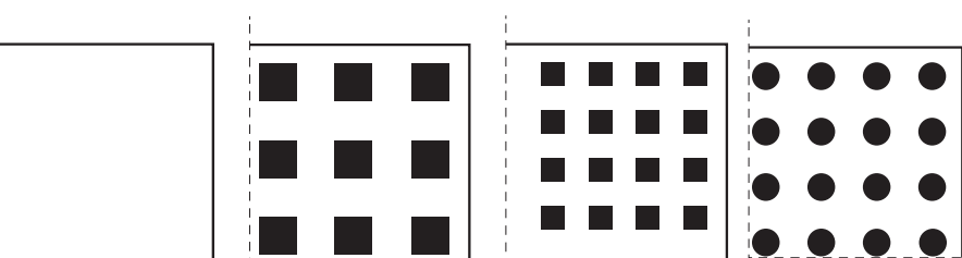
Lisse Perforation 8x8 24 % perforation Perforation 5x5 23 % perforation Perforation Ø6 17 % perforation
