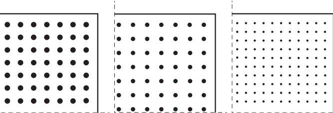
Perforation Ø2,5 U | 13 % perforation M | 25 % perforation ML | 6 % perforation Perforation Ø2 U | 9 % perforation M | 19 % perforation Perforation Ø1,5 U | 11 % perforation ML | 5 % perforation
