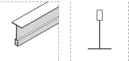
Ossature T- 24 x 38
